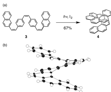
Figure 1. One-step synthesis of [9]helicene ( 4 ) from [2] + [1] + [1] + [2] precursor 3 . a) Reaction scheme. b) X-ray crystal structure of 4 (ORTEP, thermal ellipsoids set at 50% probability). Only one enantiomer is observed in the crystal structure because of spontaneous resolution into the P2_1 chiral space group. The absolute stereochemistry was not determined from the data and the M form is tentatively shown.
